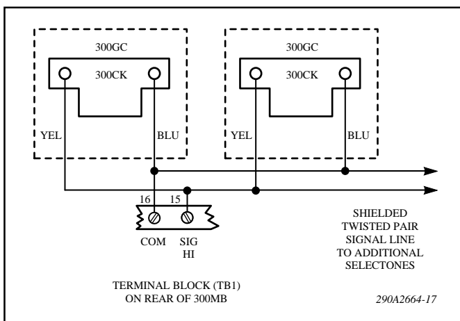
Figure 3-3. 300CK Connections.
