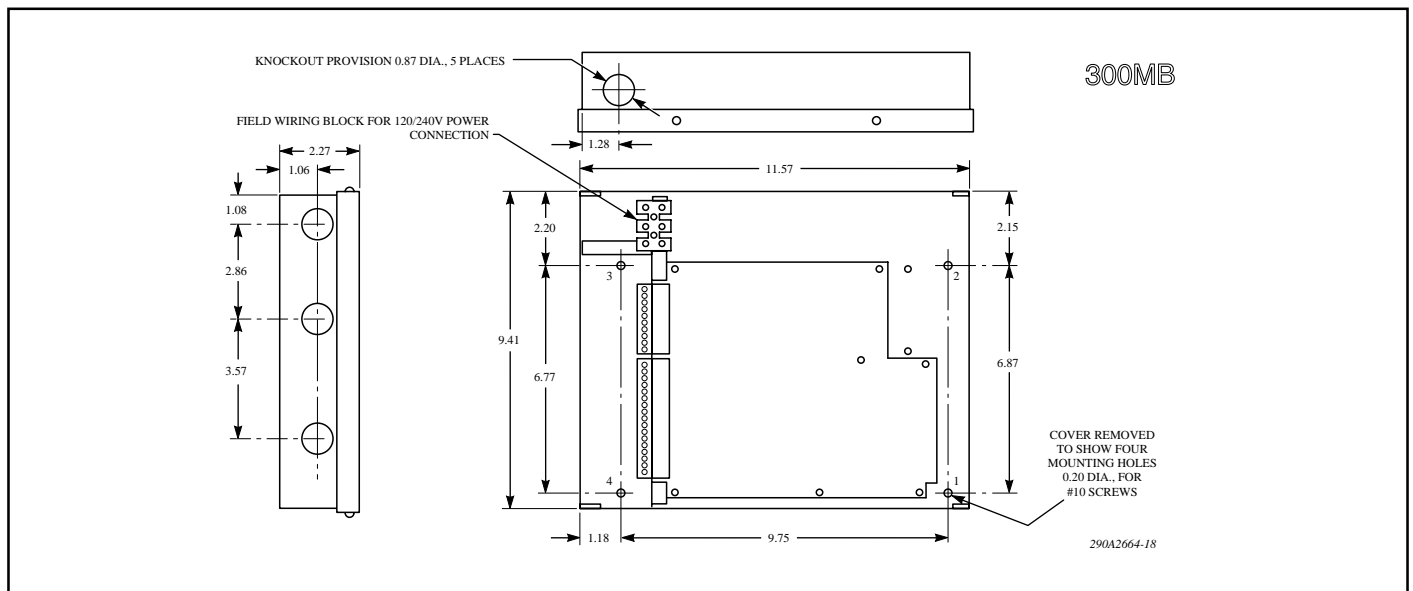
Figure 1-2. Mounting Holes and Dimensions.
