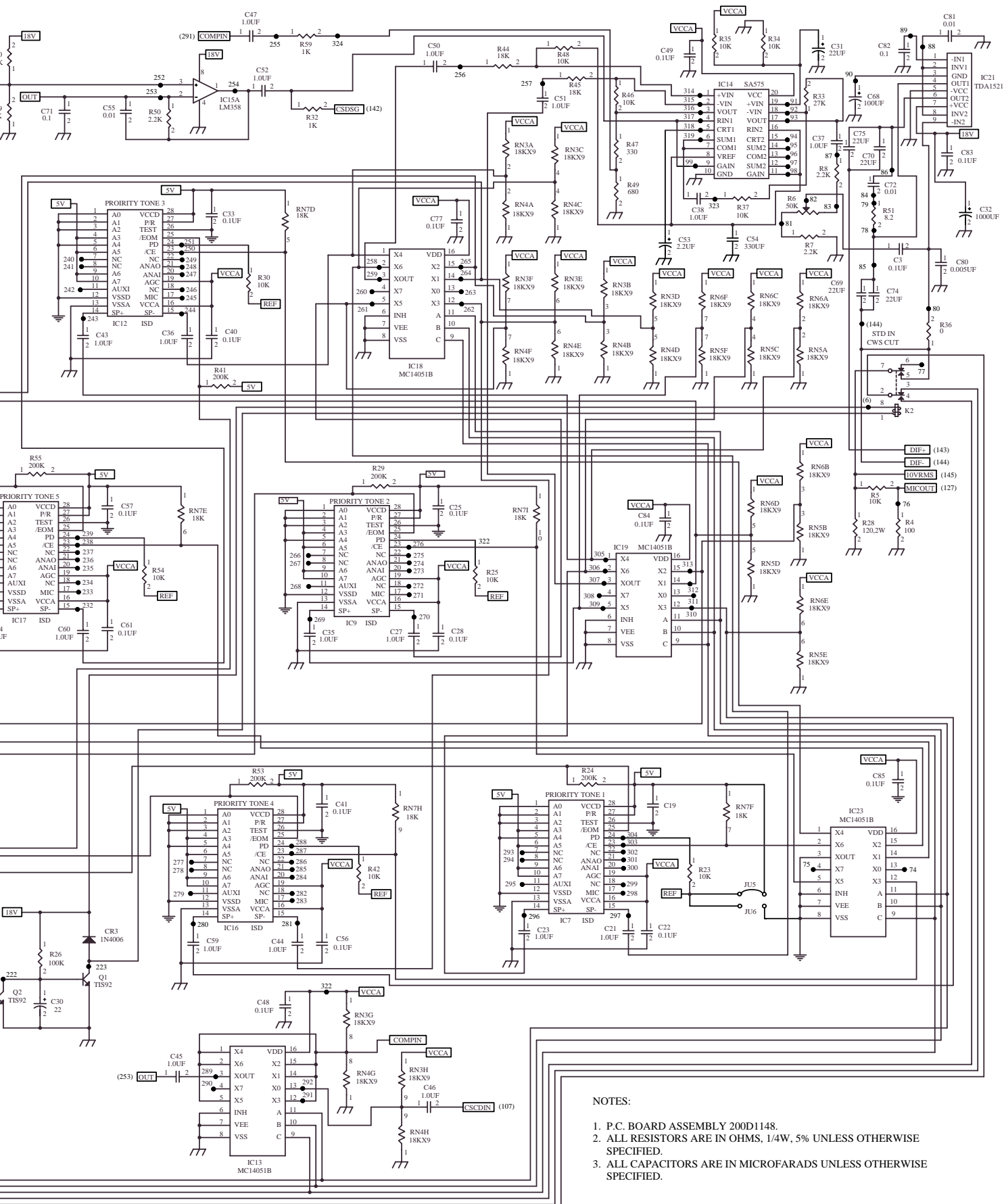
Figure 4-1. Model 300MB Schematic Diagram.
