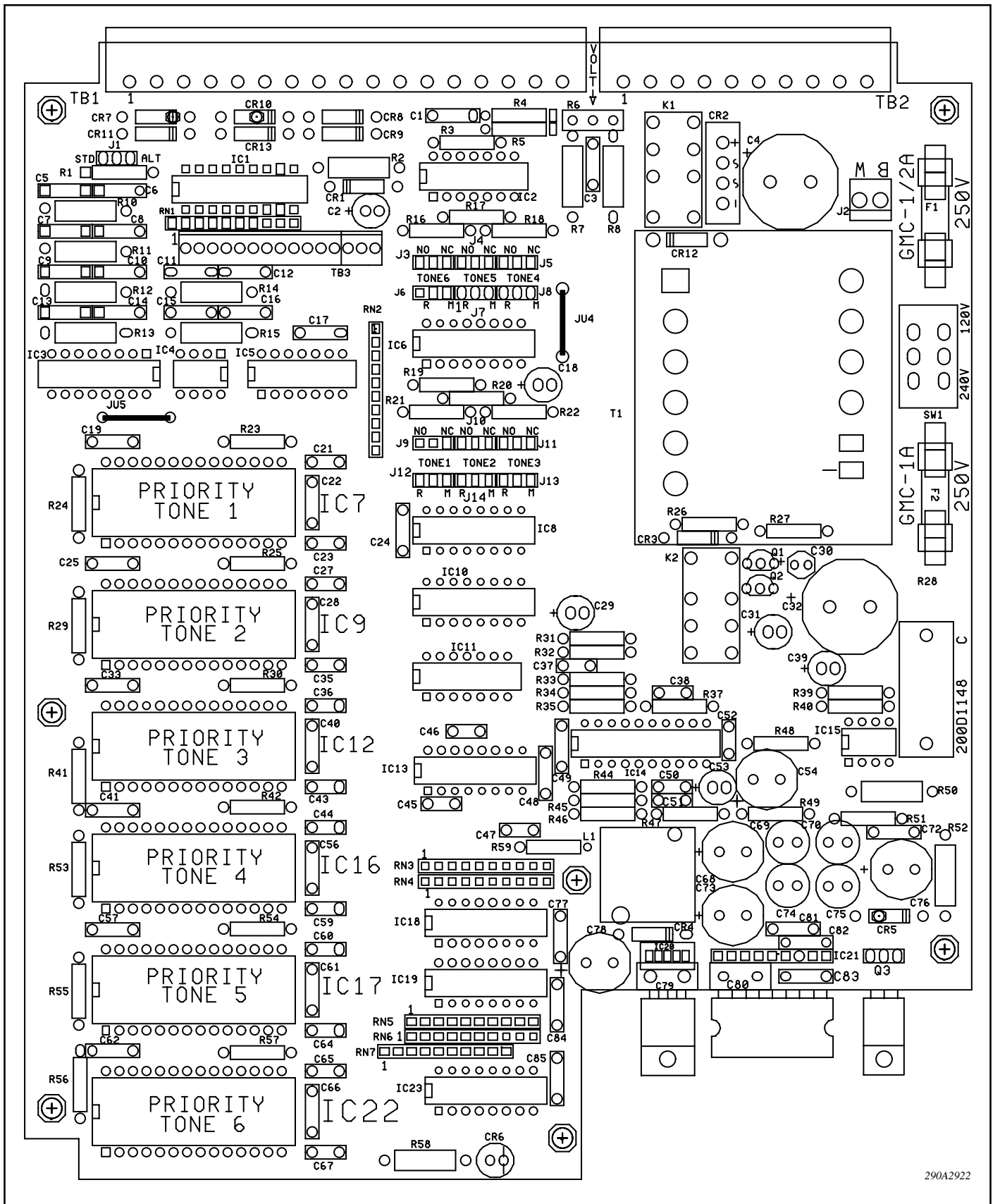
Figure 1-3. Model 300MB Series B Mother Board.
