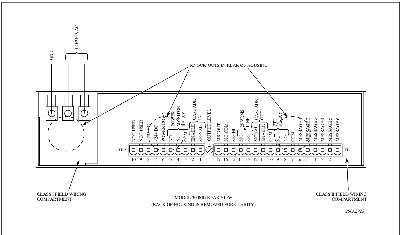
Figure 3-1. Model 300MB Rear View.
