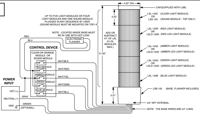
AN INSTALLATION SCENARIO SHOWING THE RED AND GREEN LIGHT MODULES WIRED TO A FLASHER. THE OTHER LIGHT MODULES ARE STEADY BURNING WHEN TURNED ON. THE FLASHER IS FOR USE WITH 120VAC LIGHT MODULES ONLY. THE SOUND MODULE CANNOT BE WIRED TO THE FLASHER. 29042856F
