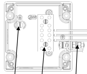
Internal Earth terminals
