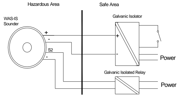
Fig 8 Multi stage alarm using galvanic isolated relays
