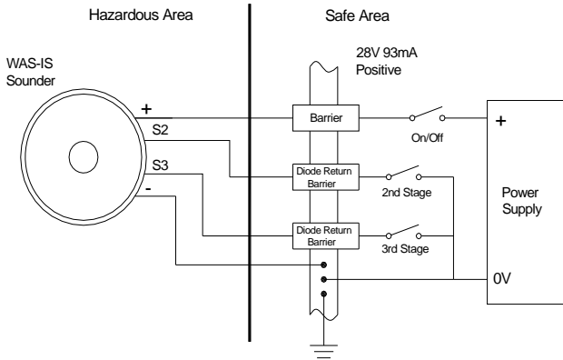
Fig 6 Multi stage alarm using Zener barriers.
