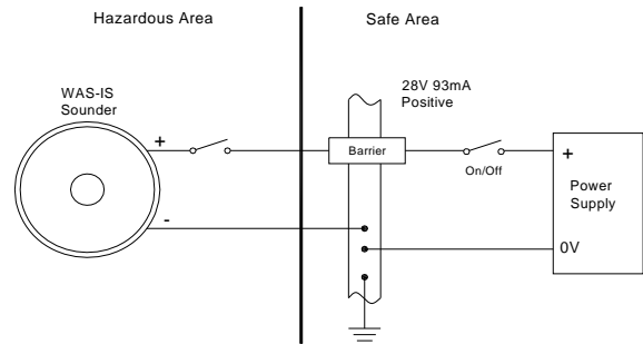
Fig 4 Single stage alarm using single channel barrier.
