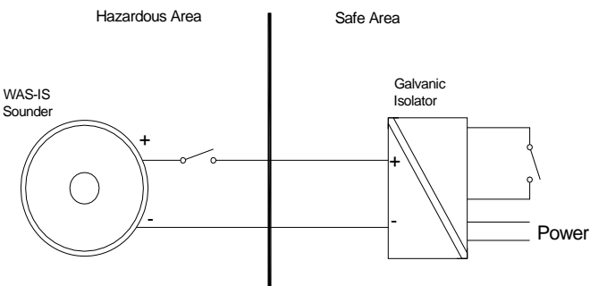
Fig 7 Single stage alarm using galvanic isolator.
